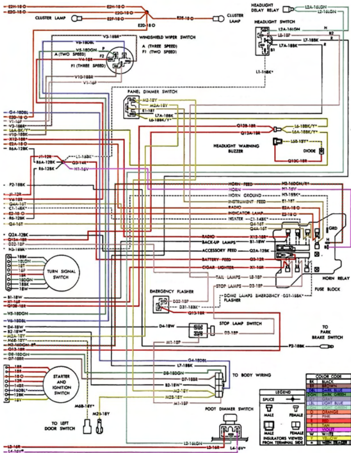
Fig. 28—Instrument Panel Wiring Diagram (Rallye Cluster)—Barracuda
