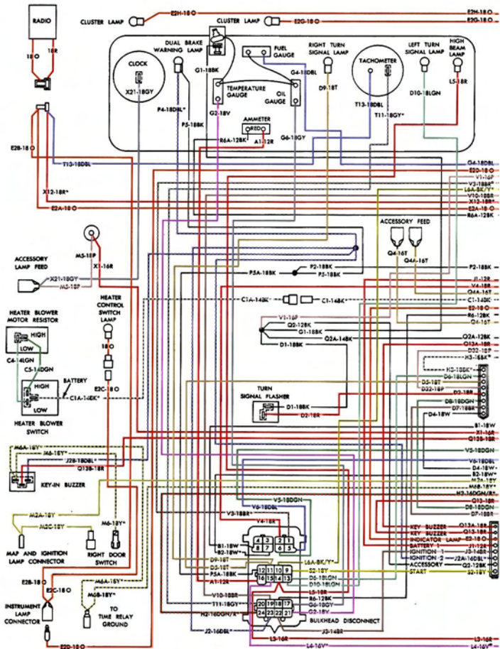
Fig. 28—Instrument Panel Wiring Diagram (Rallye Cluster)—Barracuda
