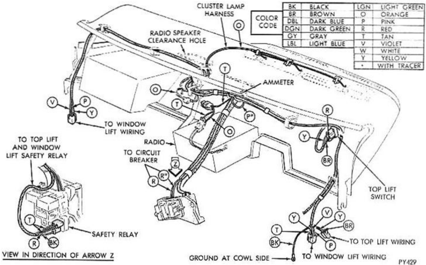
Fig. 21—Top Lift, Window Lift and Cluster Lamps Wiring—Barracuda
