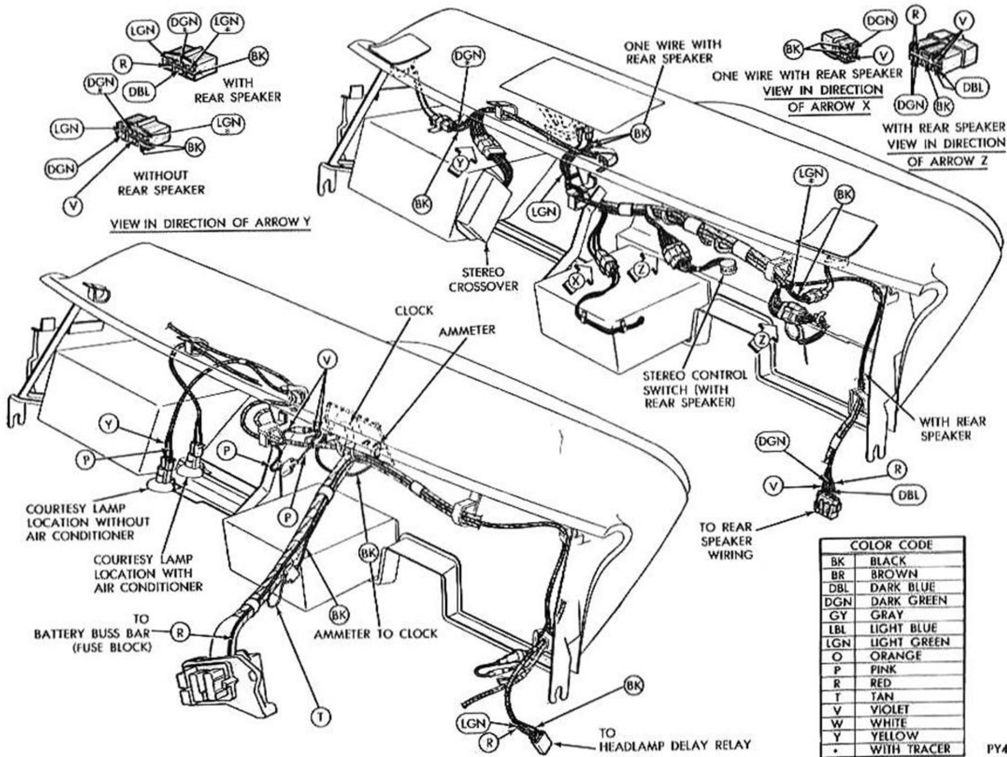
Fig. 16—Stereo, Clock, Courtesy Lamp and Headlamp Delay Relay Wiring—Barracuda
