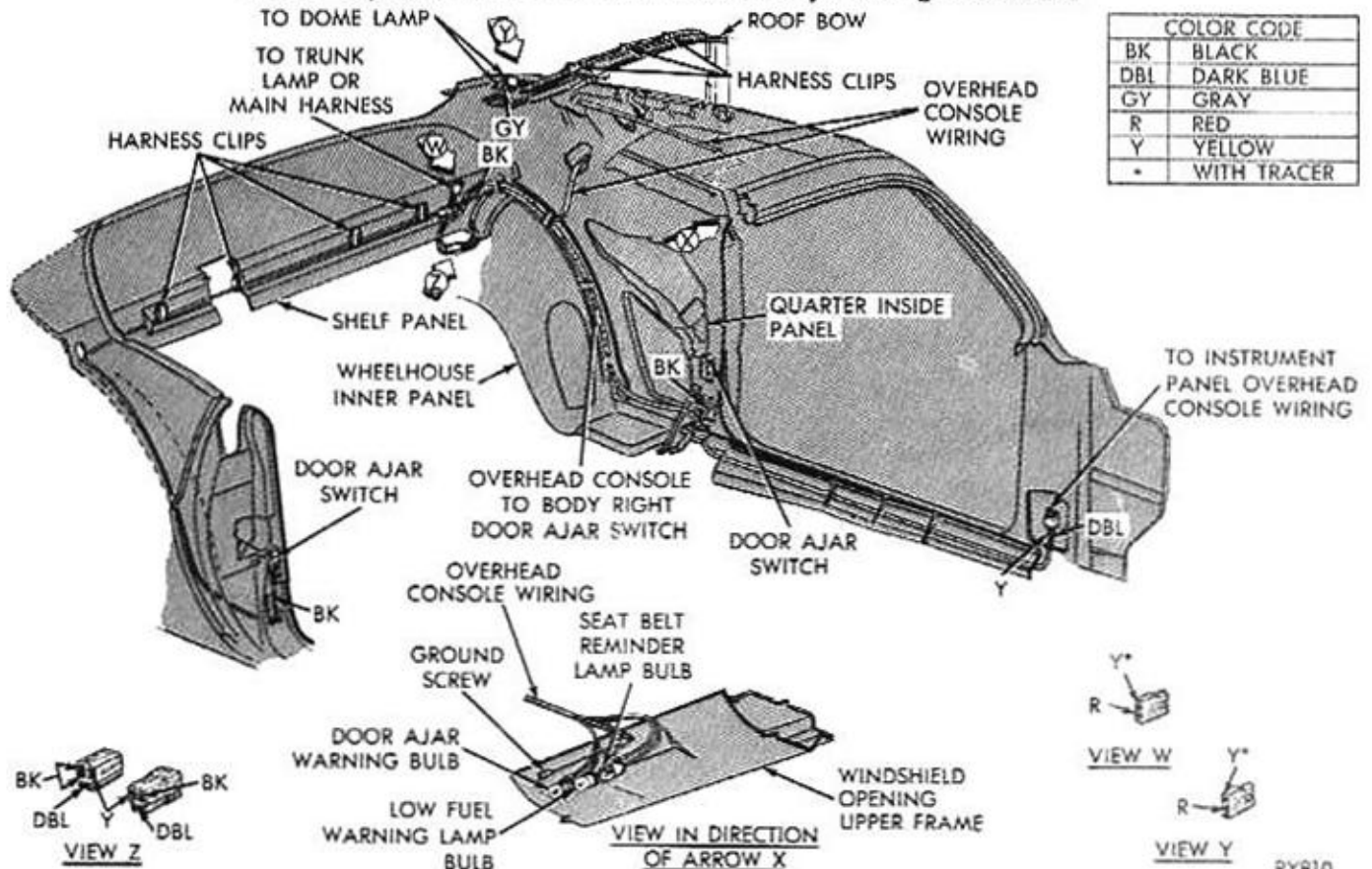
Fig. 22—Overhead Console Wiring—Barracuda
