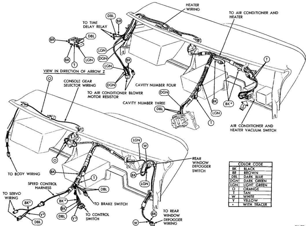
Fig. 1—Air Conditioner, Heater, Rear Window Defogger, Speed Control and Console Gear Selector Wiring—Barracuda
