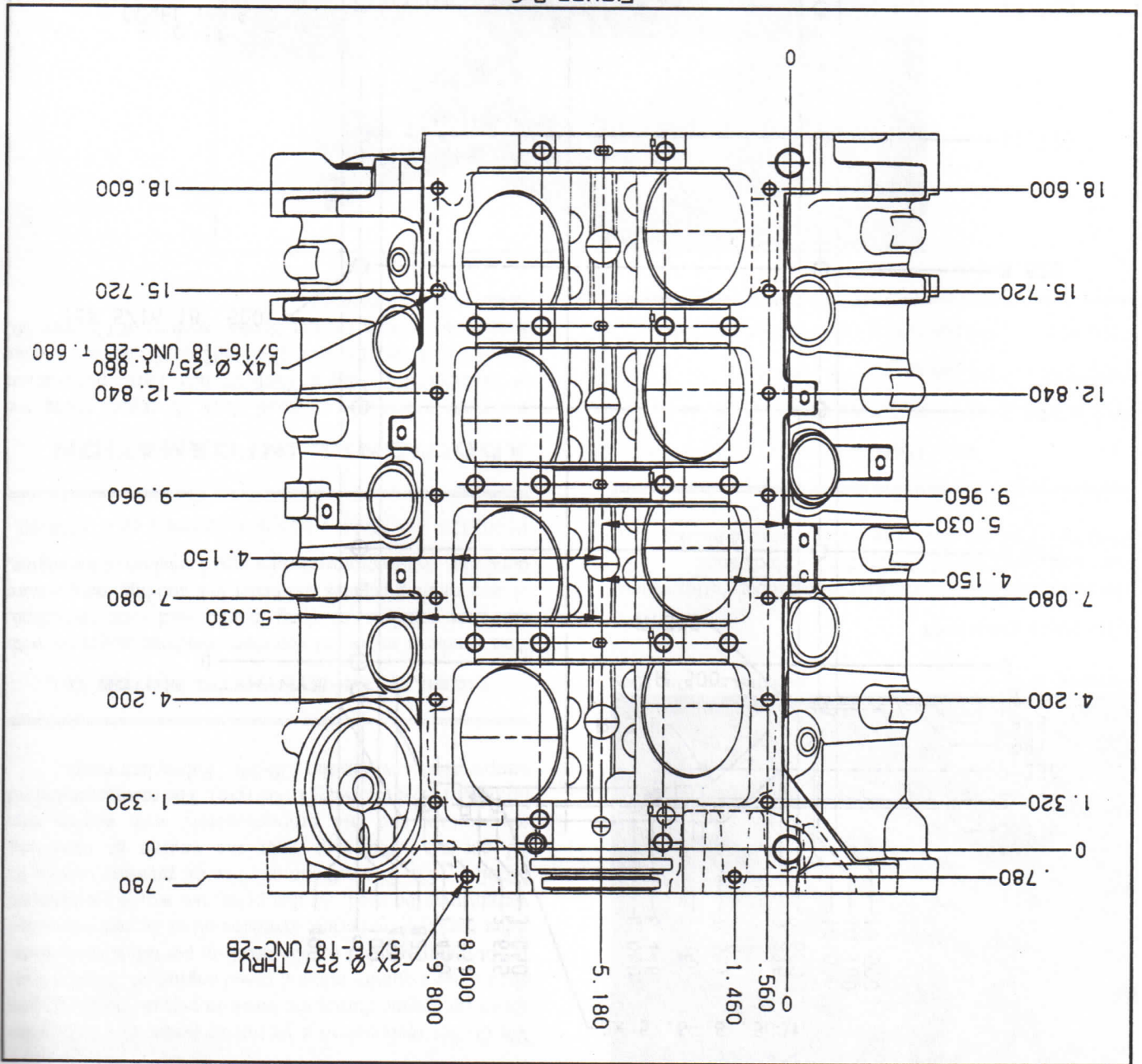
FIGURE 2-6 R3 BLOCK OIL PAN ATTACHMENT BOLT HOLES
