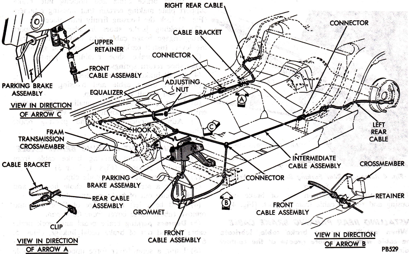
Fig. 2 Parking Brake Cable Routing (Challenger and Coronet Models)
