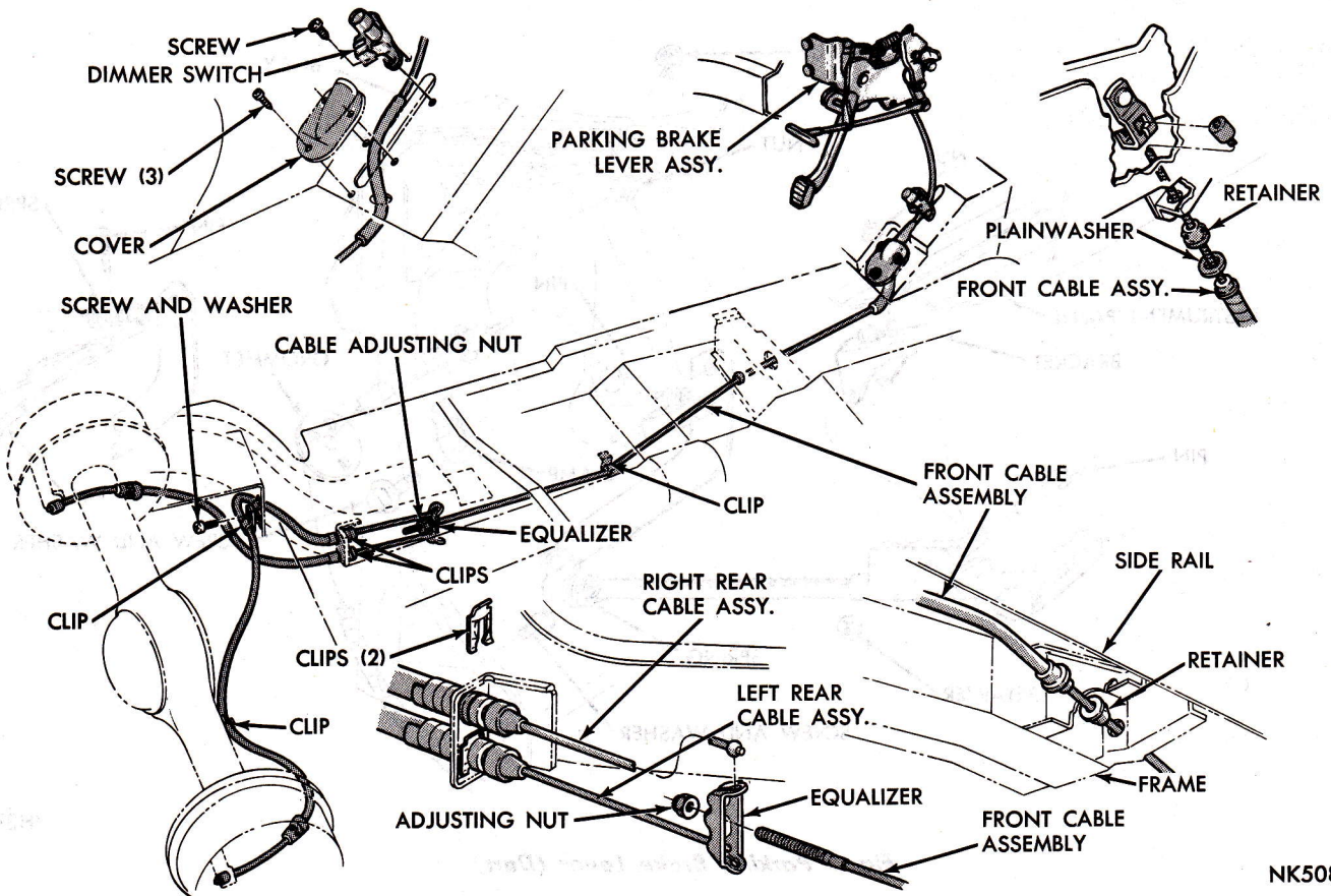
Fig. 3 Parking Brake Cable Routing (Polaris Monaco)
