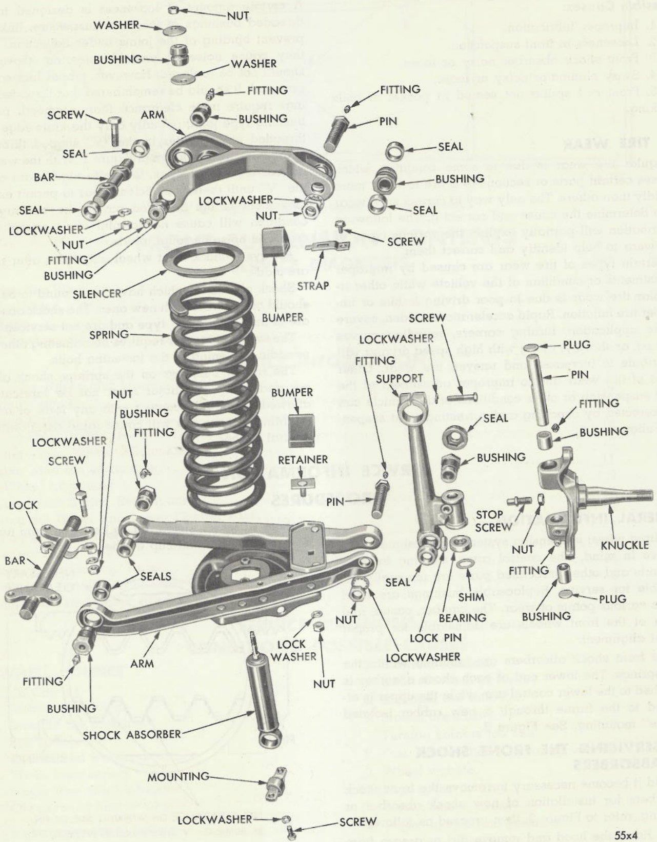
Fig. 2—Front Suspension (Exploded View)
