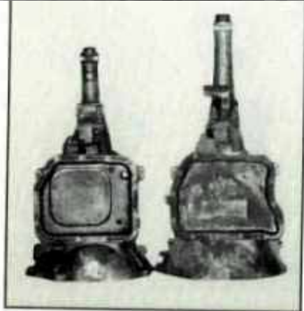
The A-727 transmission on the right is nearly 4 inches longer than the A-904 on the left. Also, note the difference in the shape of the pans. The A-727 has a hump on the passenger's side near the front.
