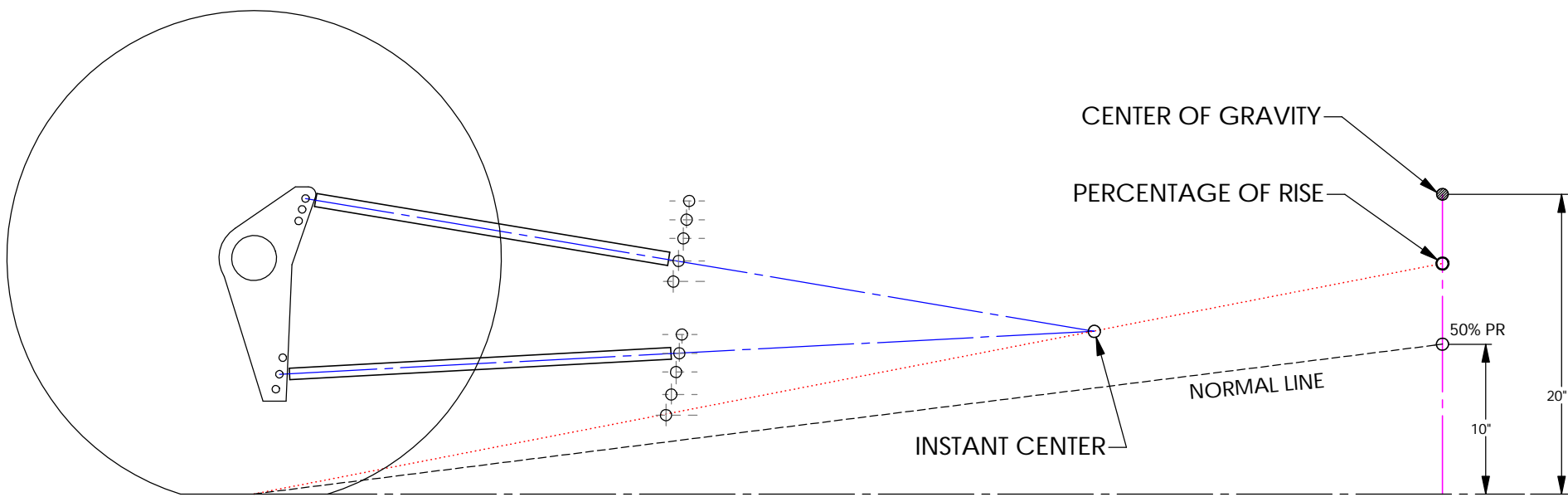
4-LINK SUSPENSION
