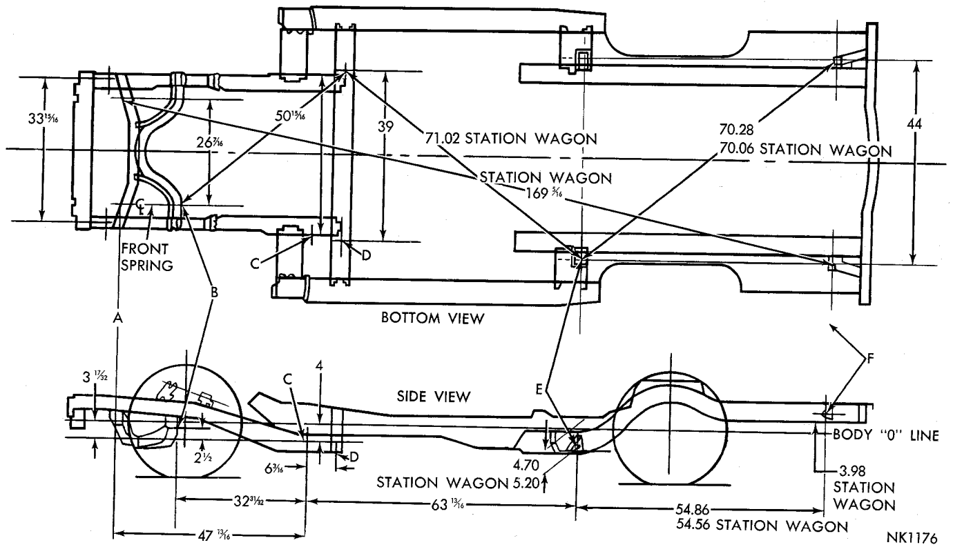
Fig. 198—Body Frame Dimensions (AR Models)
